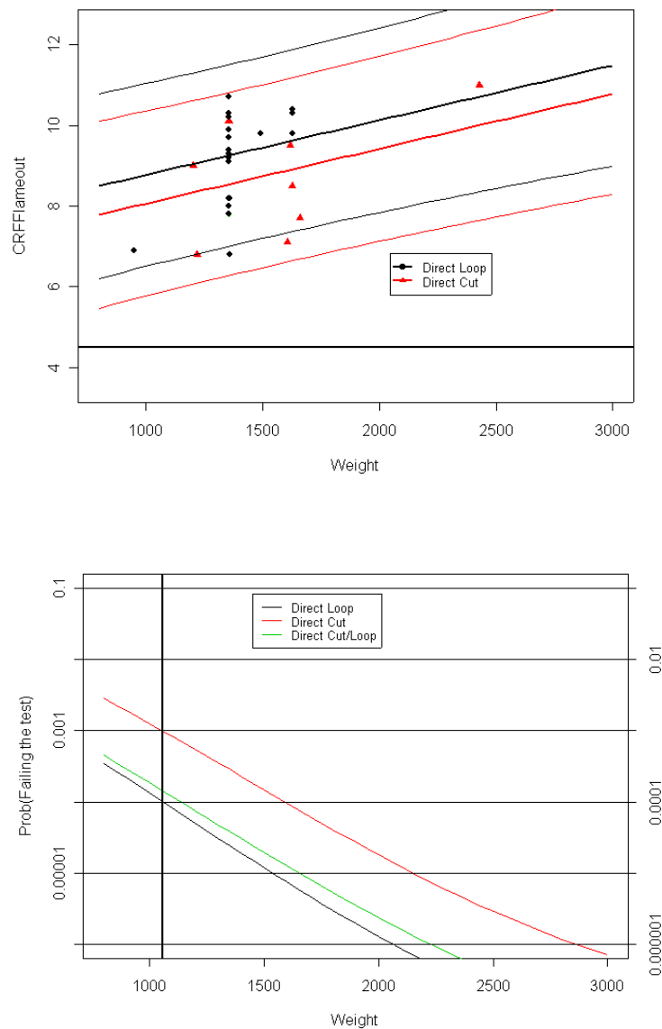
Figure 7.7: CRFFlameout vs Weight for Direct Stick and probability of failing the CRFFlameout test at 4.5 kW/m 2 .
