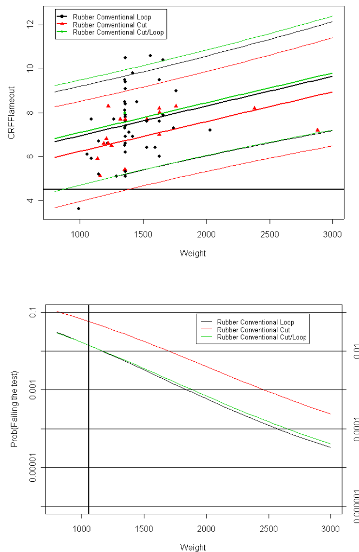
Figure 7.3: CRFFlameout vs Weight for Rubber with 95% prediction intervals; and probability of failing the CRFFlameout test at 4.5kW/m 2 .
