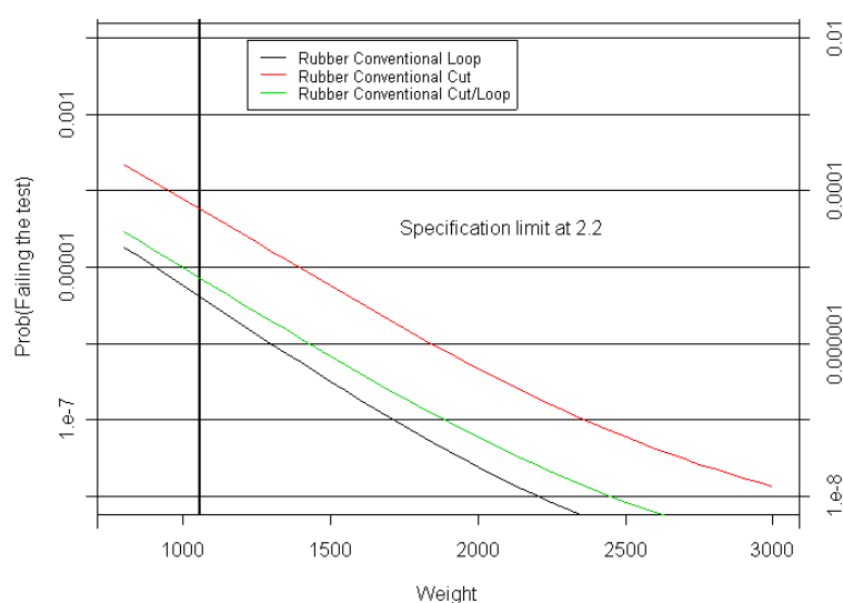
Figure 7.4: Probability of failing the CRFFlameout test at 2.2 kW/m²; Rubber
