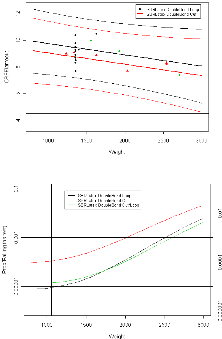
Figure 7.8: CRFFlameout vs Weight for SBR Latex and probability of failing the CRFFlameout test at 4.5 kW/m 2 .
