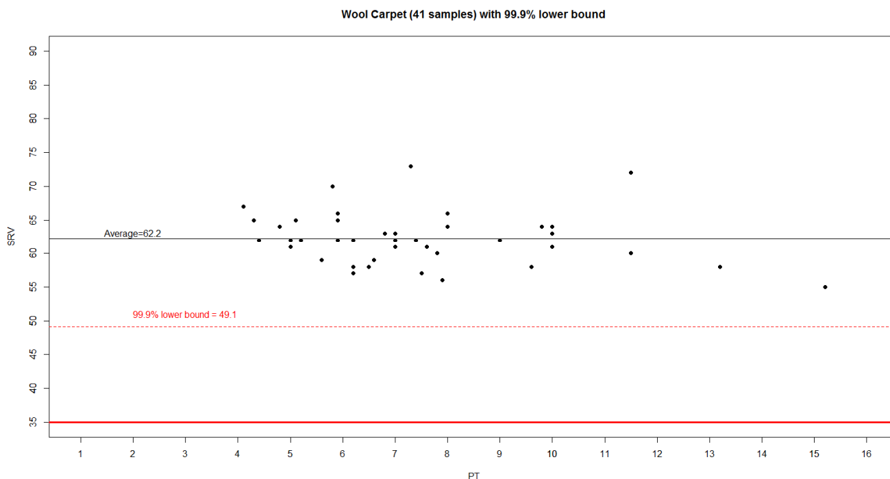
Figure 8: Modelling of Wool carpet.
