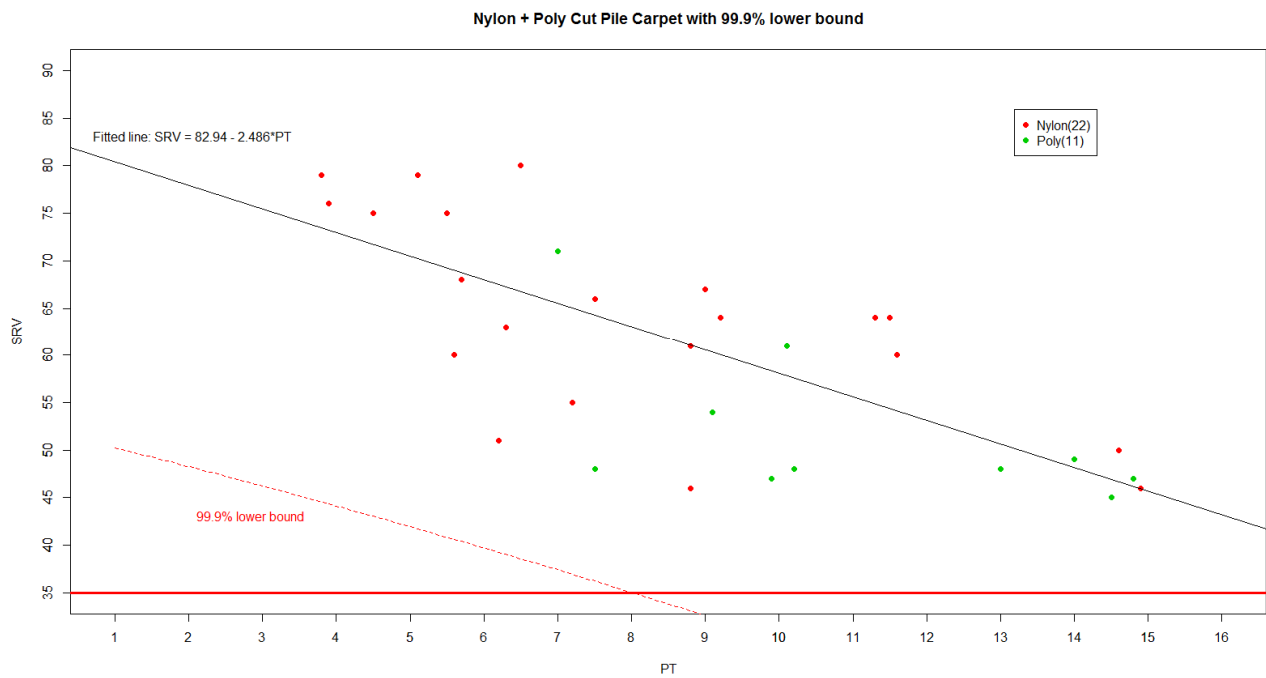
Figure 14: Modelling of Nylon cut pile and Poly Cut pile carpet.
