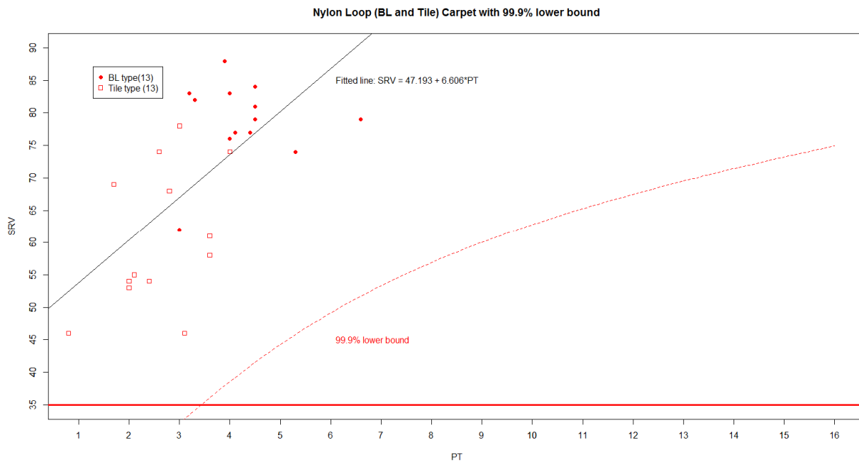
Figure 11: Modelling of Nylon Loop carpet.
